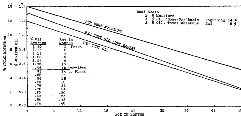
FIGURE 1. LOSS IN VOLATILE OIL OF JUNIPER BERRIES (ITALIAN) WITH AGE BY CLEVENGER METHOD (STEAM DISTILLATION)
