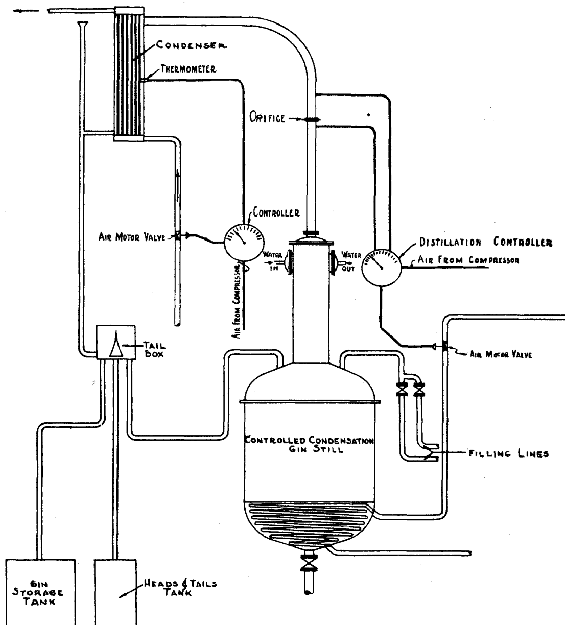
FIGURE 2. CONTROLLED CONDENSATION GIN EQUIPMENT
