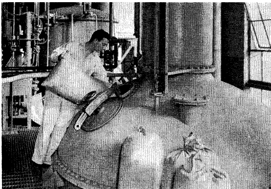
ADDING BOTANICALS TO A GIN STILL
